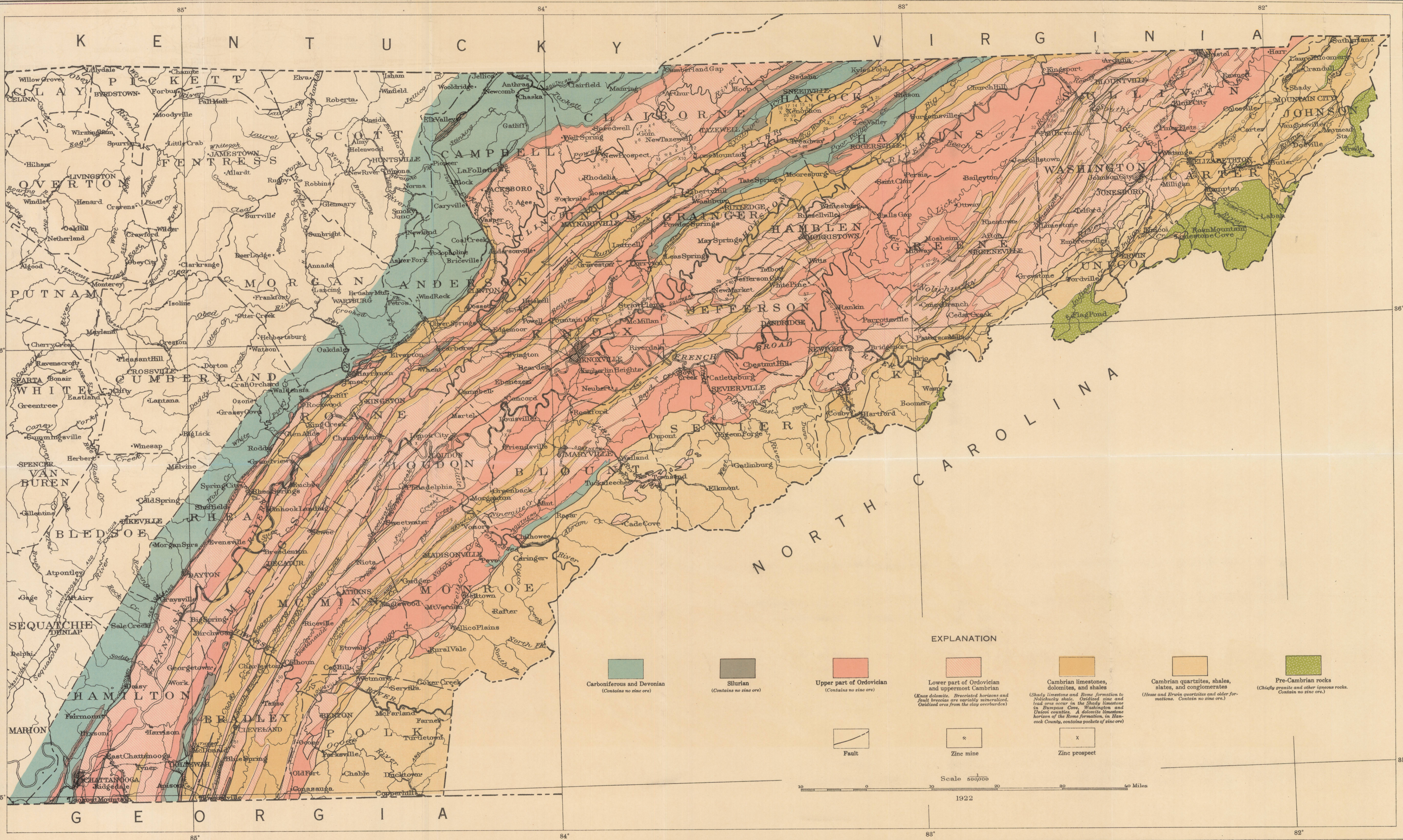
GEOLOGIC MAP OF EAST TENNESSEE, SHOWING LOCATION OF ZINC MINES AND PROSPECTS AND THEIR RELATION TO THE GEOLOGIC FORMATIONS
