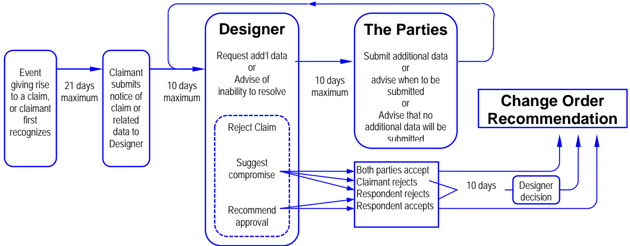
Claims Flowchart:
