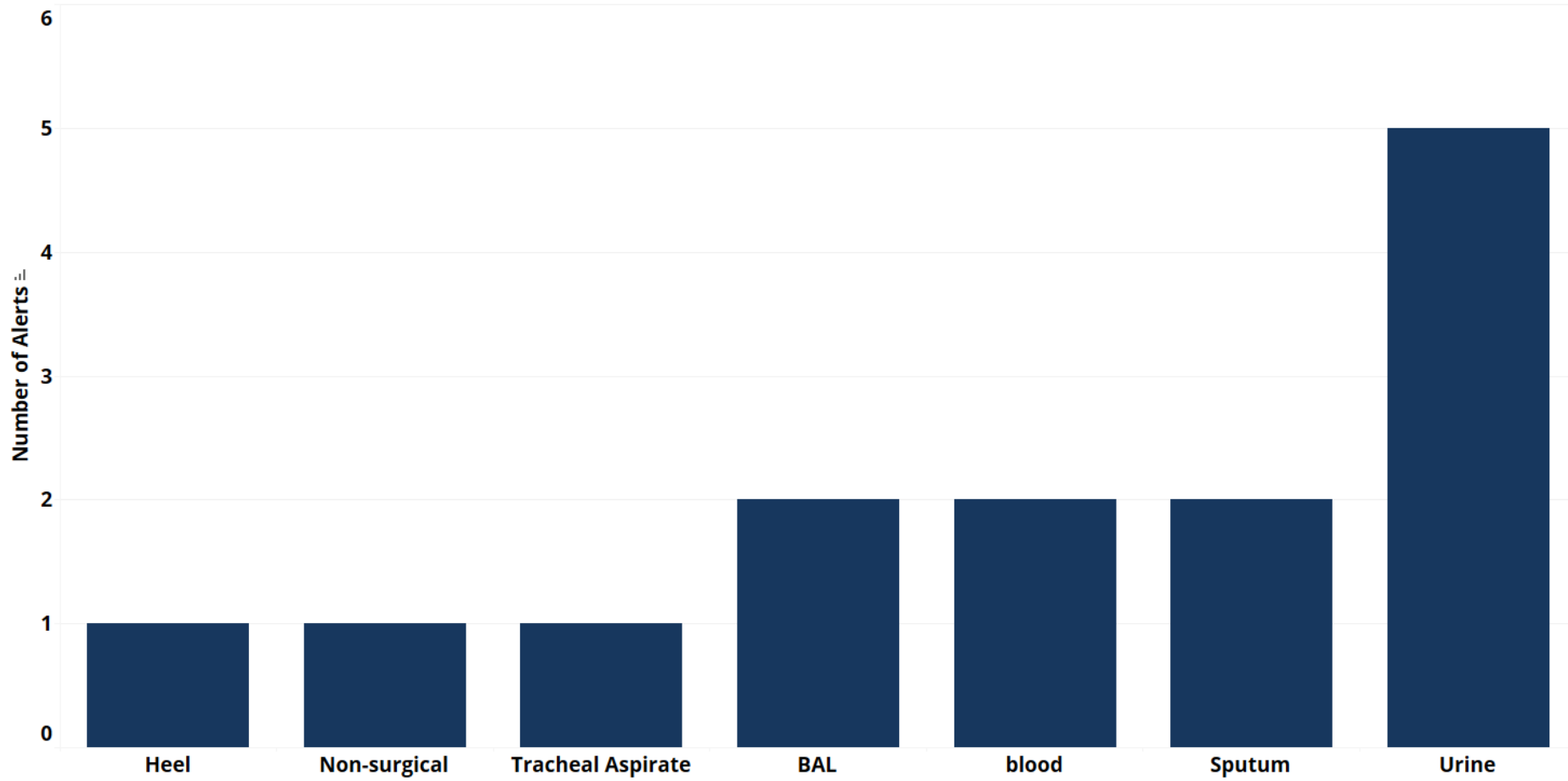
Alerts by Specimen Source (Feb.17th-March.14th)
