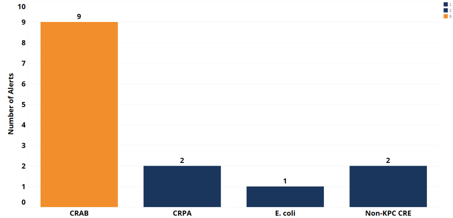
MDRO Alerts by Organism Order (Feb.17th-March.14th)
