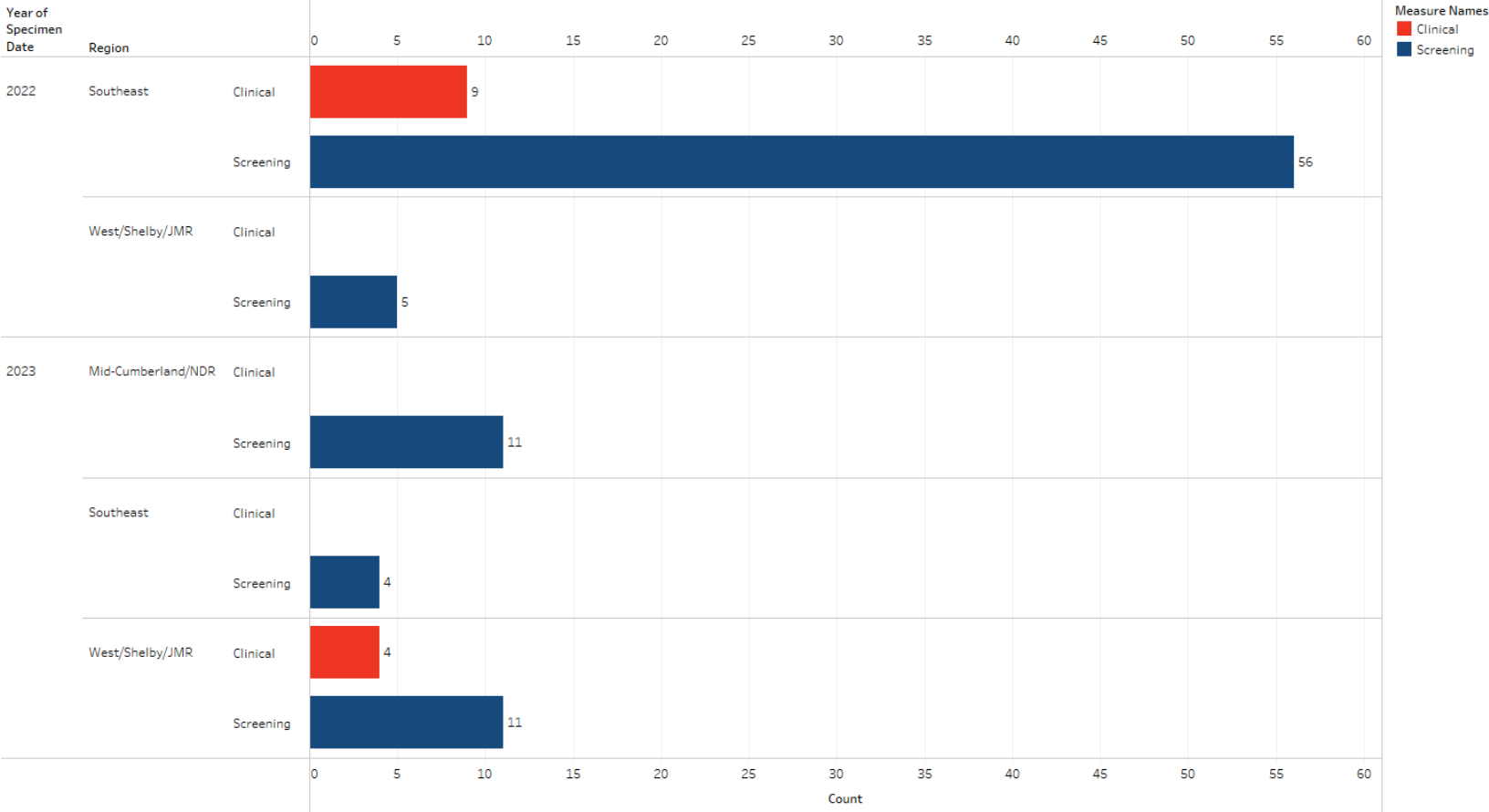
Screening vs Clinical Candida auris Cases (as of March 1, 2023)
