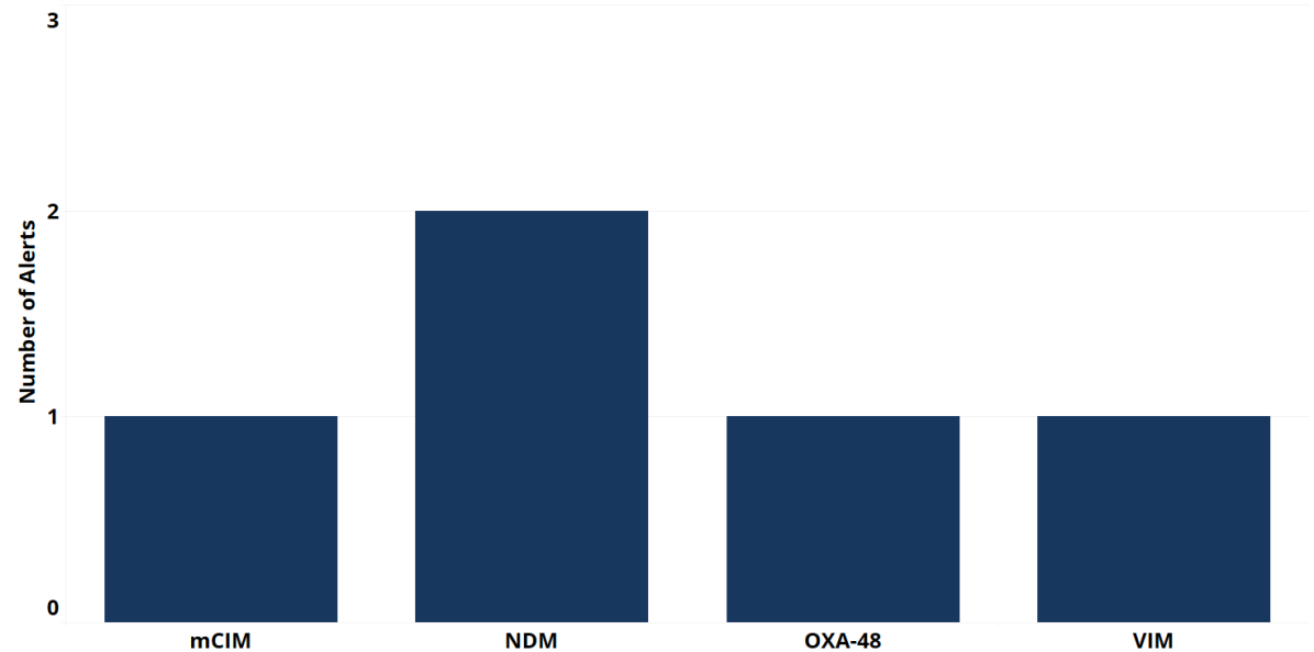
MDRO Alerts by Resistance Gene (Feb.17th-March.14th)
