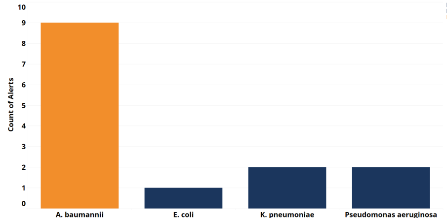
Alerts by Organism (Feb.17th-March.14th)
