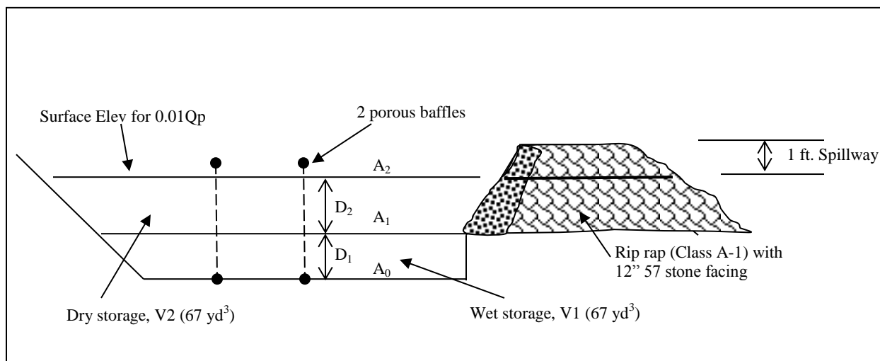
Figure 7.32-1 Sediment trap
