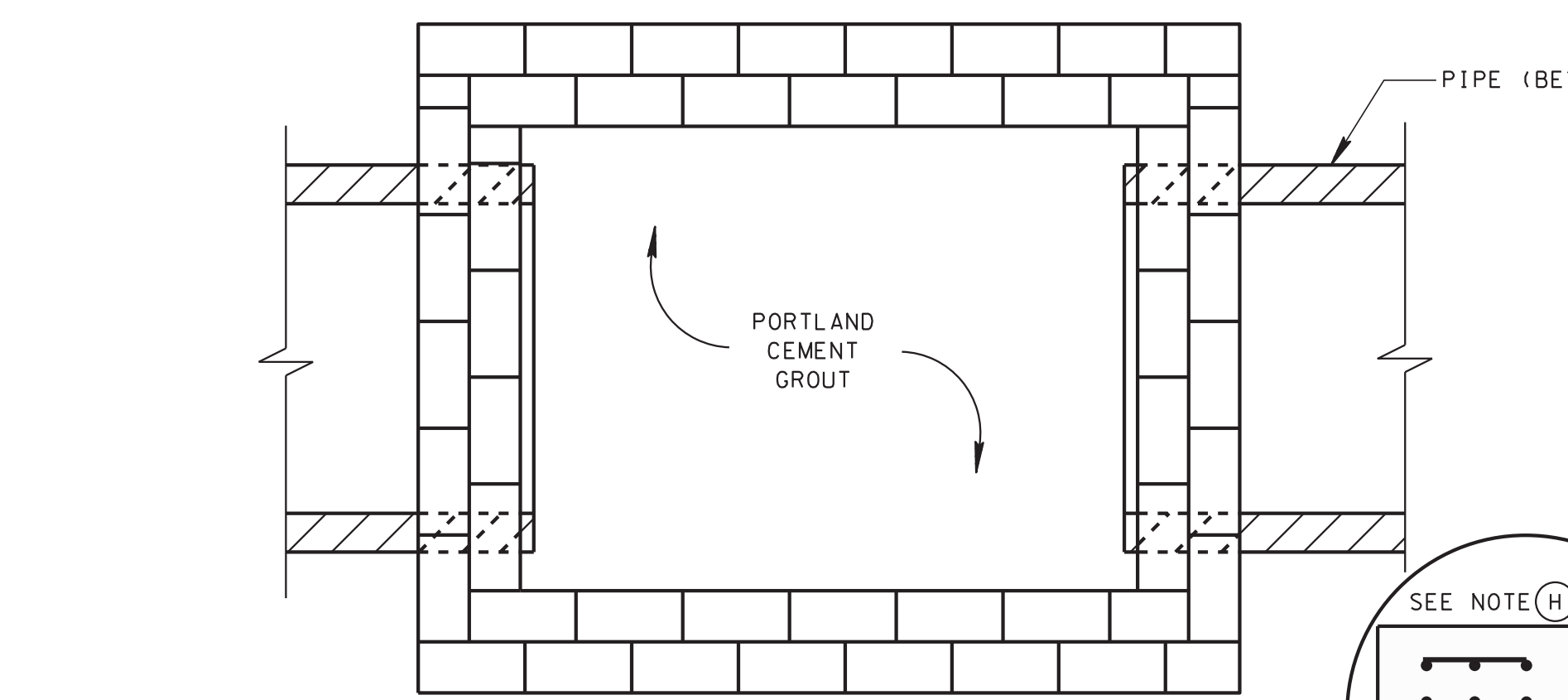
SECTION E-E
