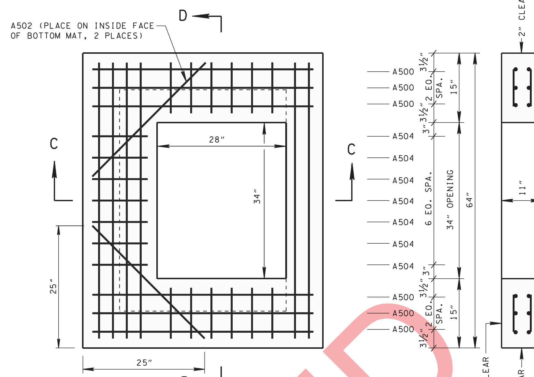
PLAN VIEW
