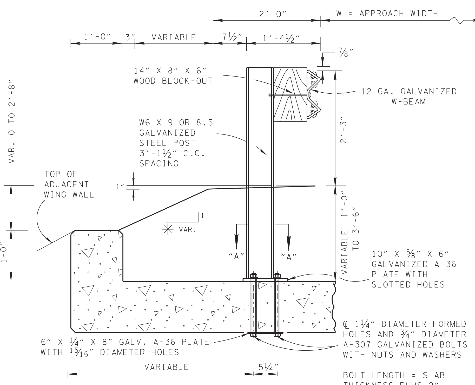
DETAIL FOR CONCRETE DECK WITH 1'-0" TO 3'-6" OF ROADWAY FILL COVER
