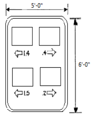
FIGURE 4: TYPICAL TRAILBLAZER BACKGROUND PANEL DETAIL
