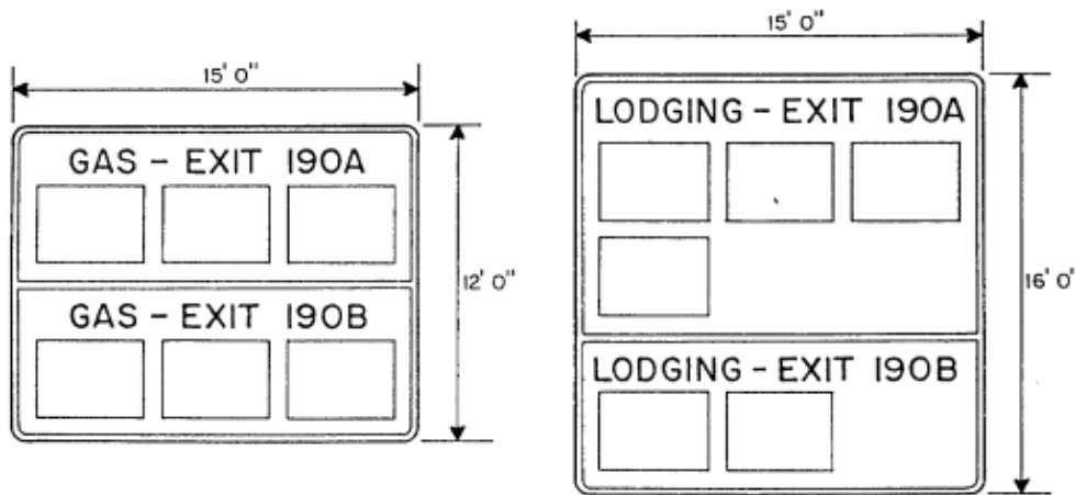
TYPICAL MAINLINE BACKGROUND SIGN PANEL DETAIL (DOUBLE EXIT RAMP INTERCHANGE)
