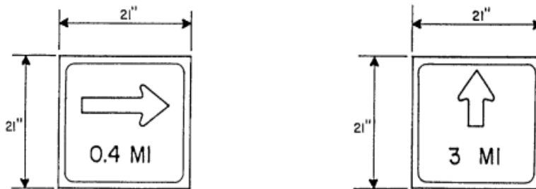
FIGURE 5: TYPICAL DIRECTION ARROW & MILEAGE DETAIL
