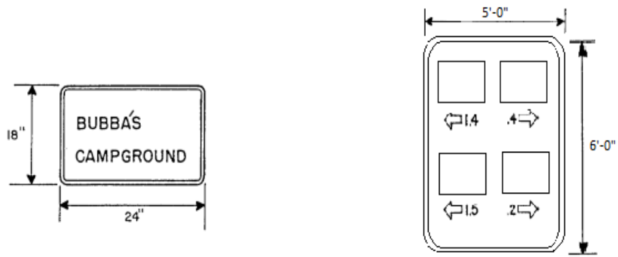
FIGURE 3: TYPICAL TRAILBLAZER SIGN DETAIL
