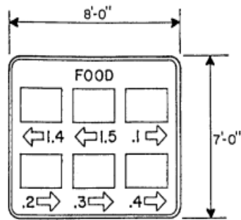
FIGURE 2: TYPICAL EXIT RAMP BACKGROUND SIGN PANEL DETAIL
