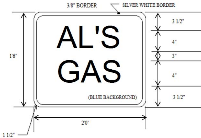
FIGURE 7: TYPICAL EXIT RAMP LOGO SIGN DETAIL (FOR ALL MOTORIST SERVICES)
