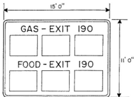
TYPICAL COMBINATION MAINLINE BACKGROUND SIGN PANEL
