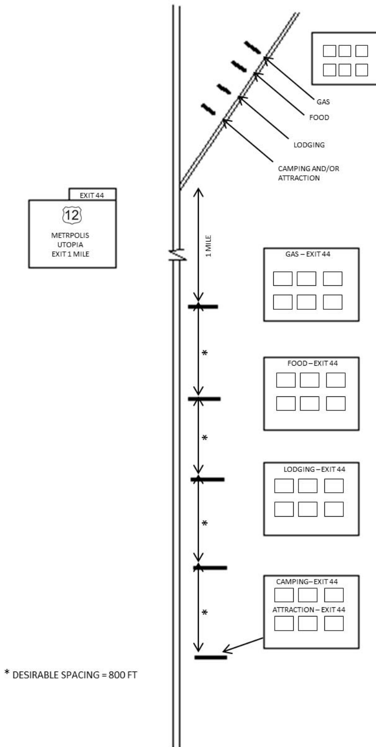
FIGURE 8: TYPICAL SIGN LOCATION DETAIL
