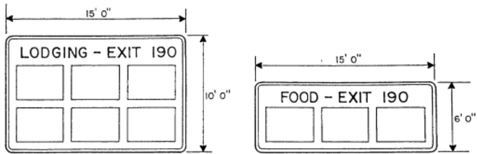
TYPICAL MAINLINE BACKGROUND SIGN PANEL DETAIL (SINGLE EXIT RAMP INTERCHANGE)
