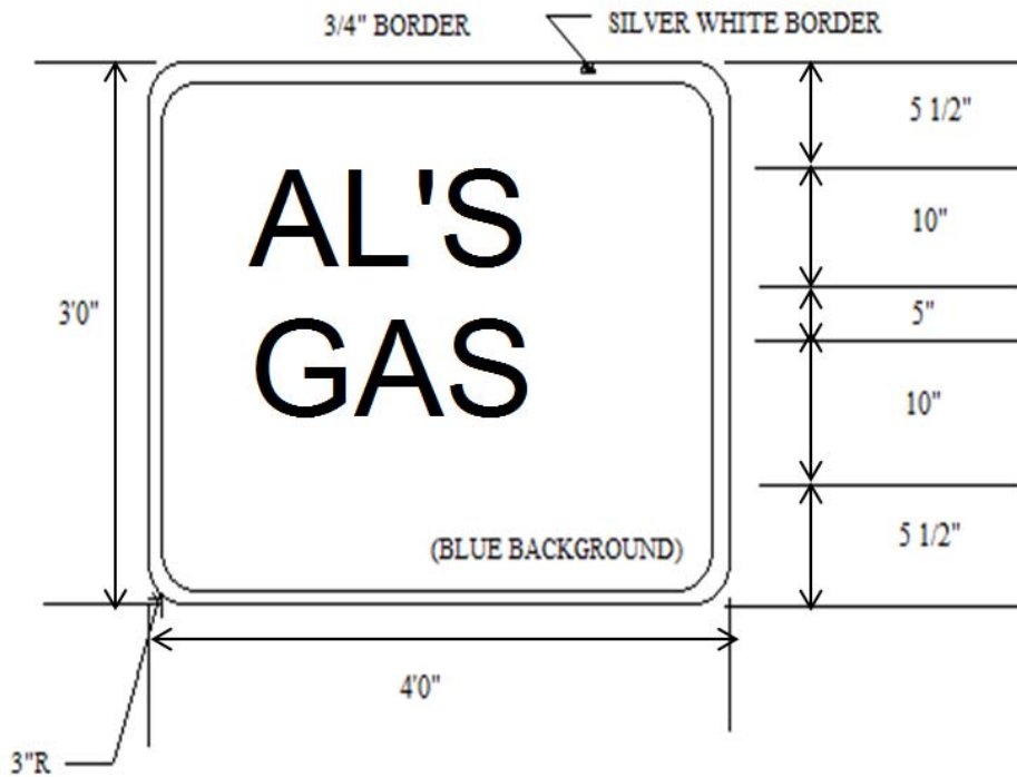
FIGURE 6: TYPICAL MAINLINE LOGO SIGN DETAIL (FOR ALL MOTORIST SERVICES)
